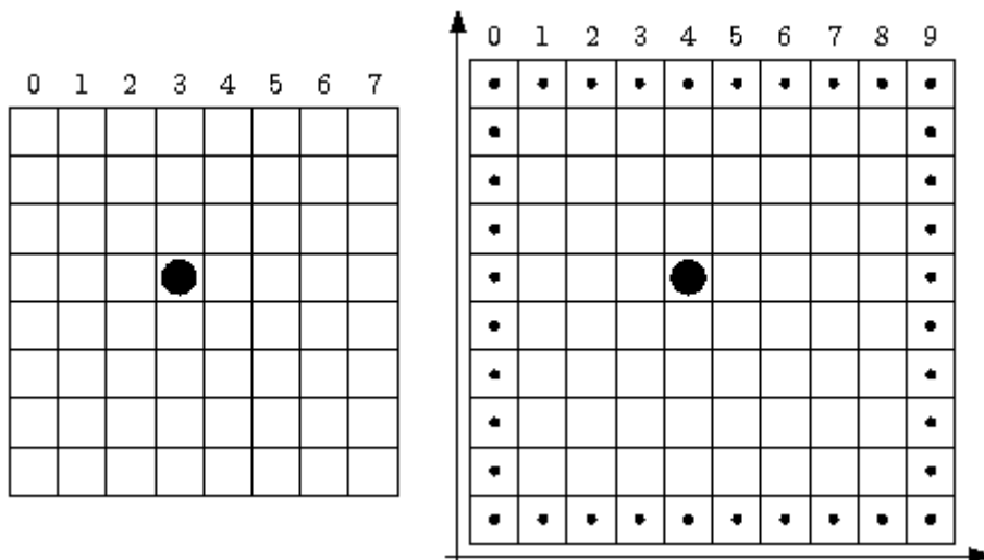
Figure 15.1 - Balle rebondissante
